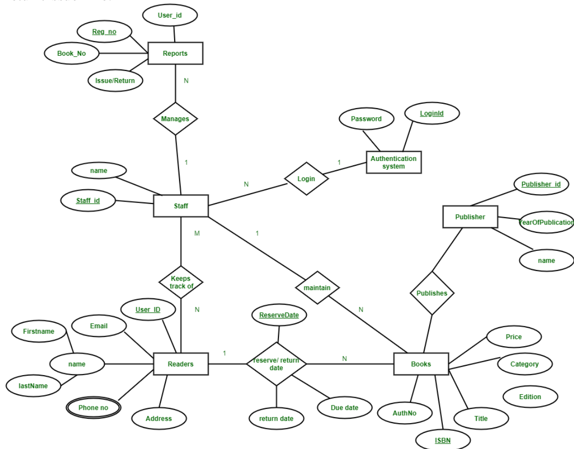
ER Diagram of Library Management System
